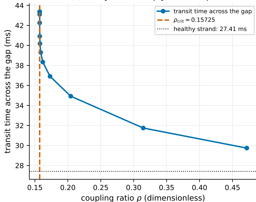
(c) Near threshold, \rho = 0.1573 : the wave stalls
