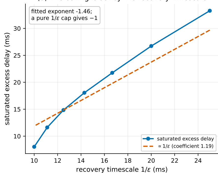
(d) The ceiling is set by the recovery timescale
