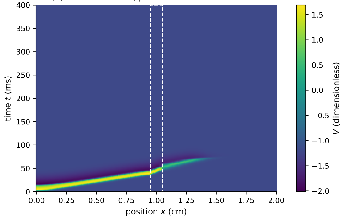
(c) Near threshold, \rho = 0.1573 : the wave stalls
