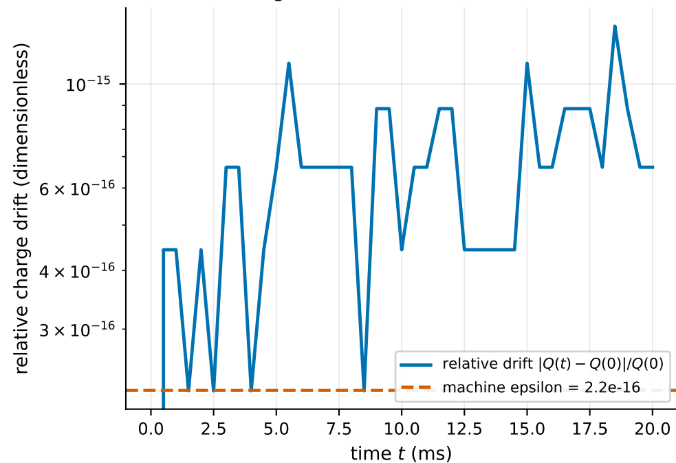
(c) Charge conservation with sealed ends
