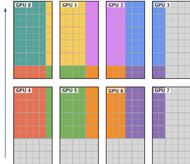
(c) Compact valid rows upward
