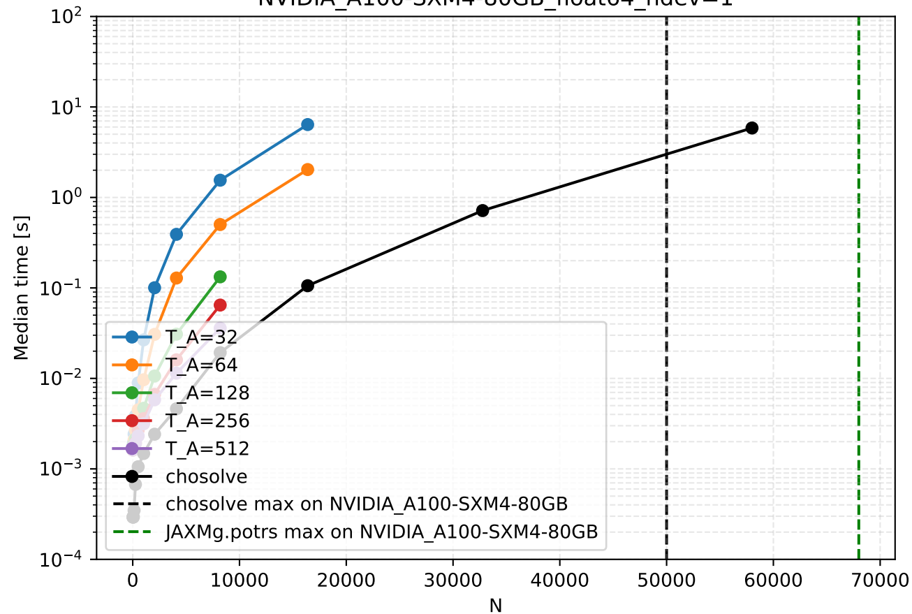
NVIDIA_A100-SXM4-80GB_float64_nde=1
