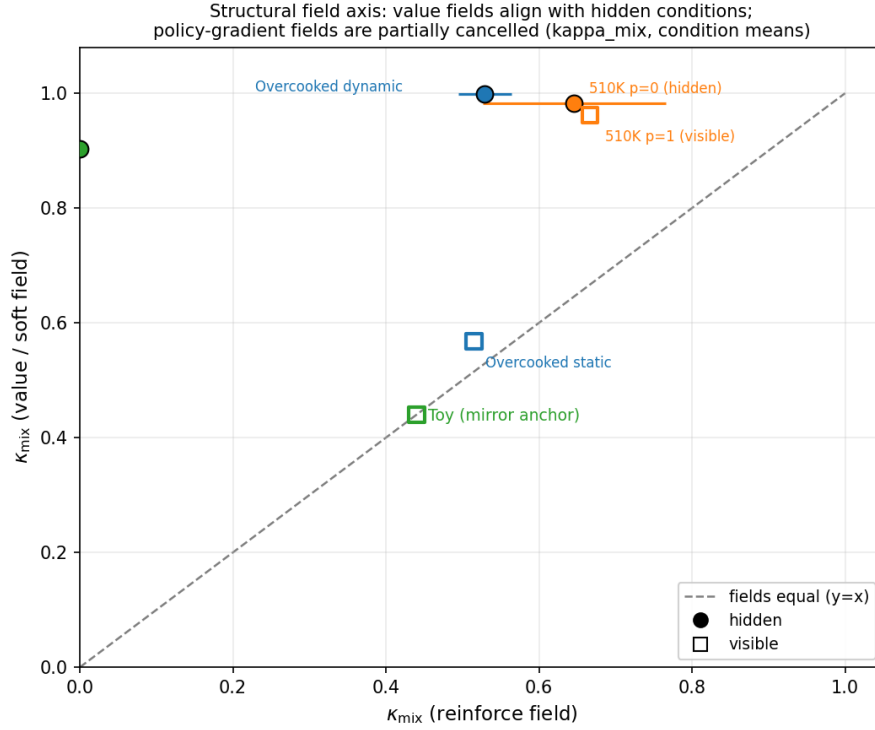
Figure 1: Structural field axis under \kappa_{\text{mix}} (condition means). Value fields stay above the diagonal; policy-gradient fields are partially cancelled (Overcooked near 0.5, 510K near 0.65 with a large seed spread). The mirror-bandit point is an exact anchor, not a real environment.
