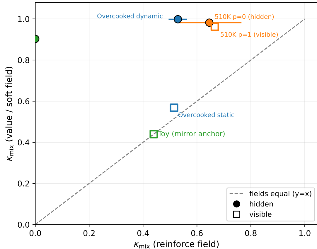
Retention alone: no condition-contrast information
