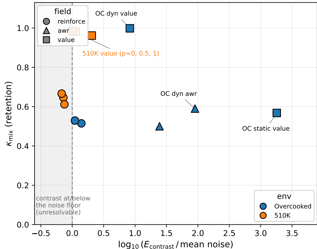
Joint read: retention vs. resolvable contrast
