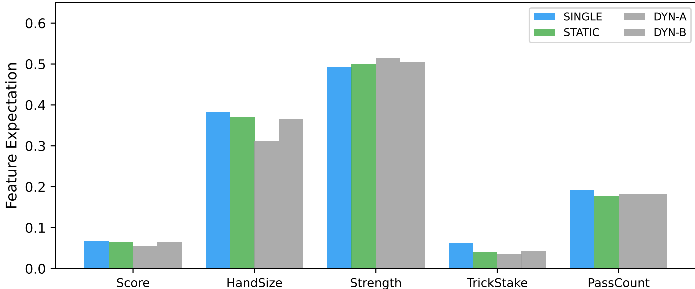
Feature Profiles of Self-Play Trained Policies
