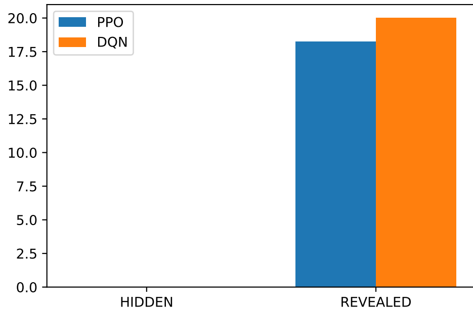
Average Reward
