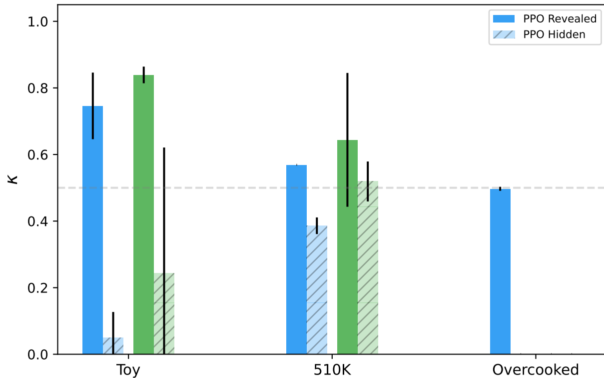
Policy-Gradient Methods
