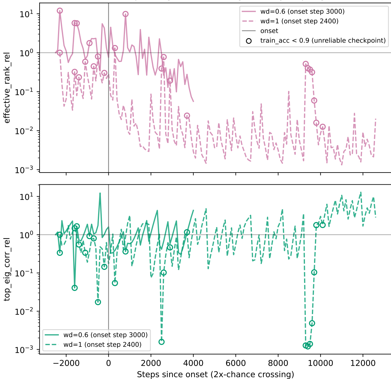
Effective-rank collapse aligns across weight decay; top-eig rise is looser
