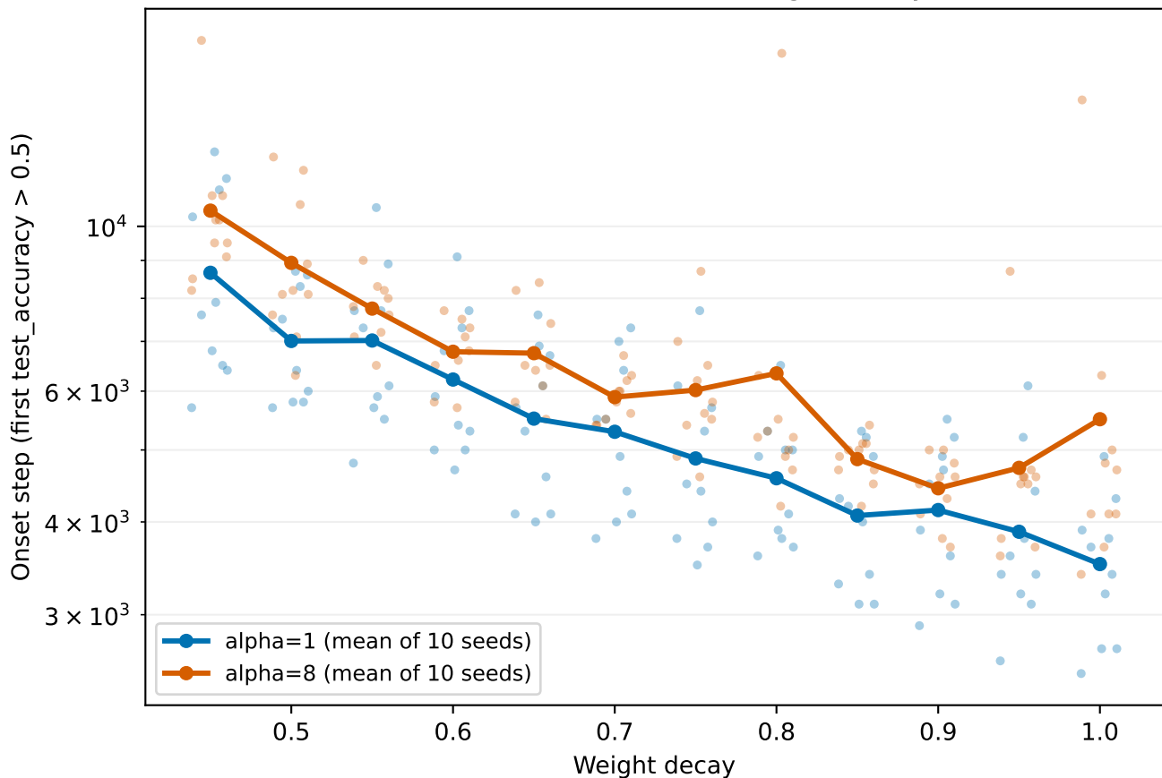
Generalization onset vs. weight decay
