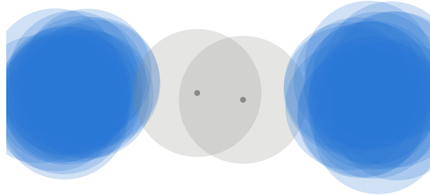
Rips, balls of radius r/2 (1 component at this r )
