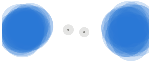
DTM 5 , balls of radius (r - w_i) + 1/2 (4 components at this r )
