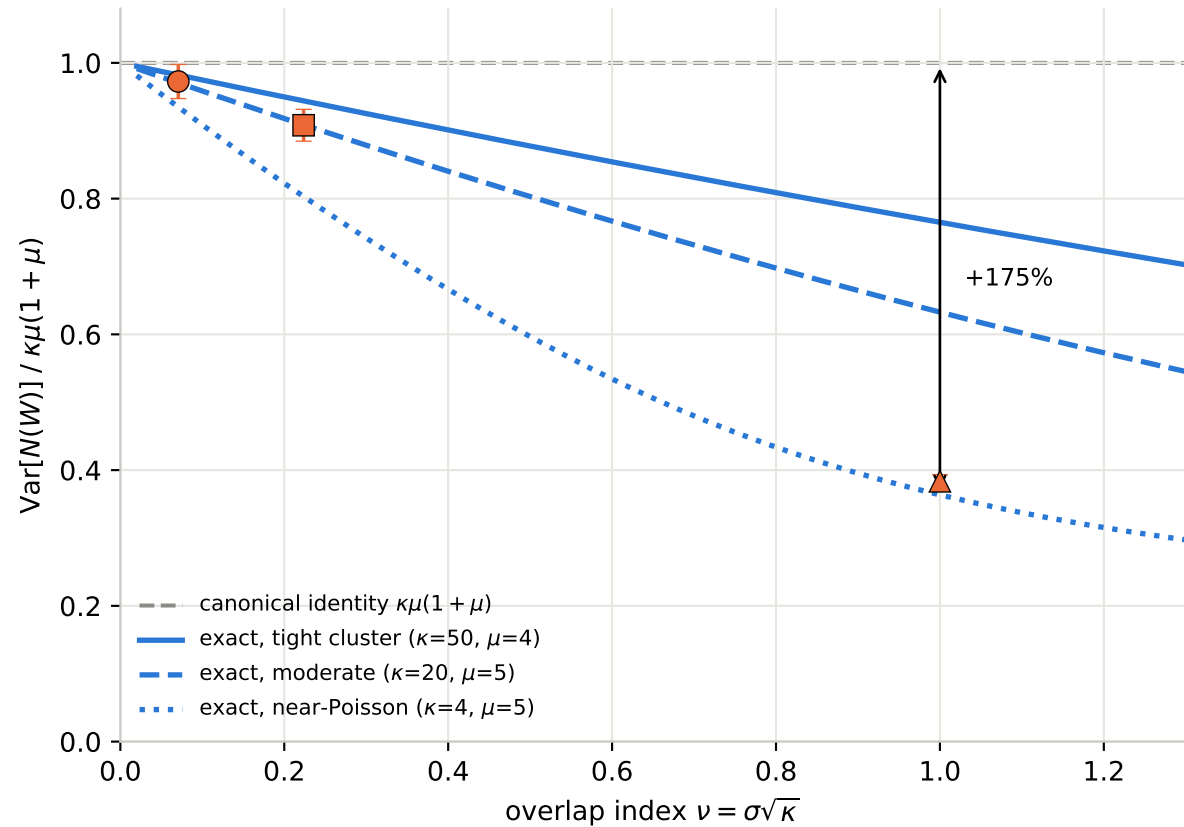
Canonical identity vs. the exact finite-window variance
