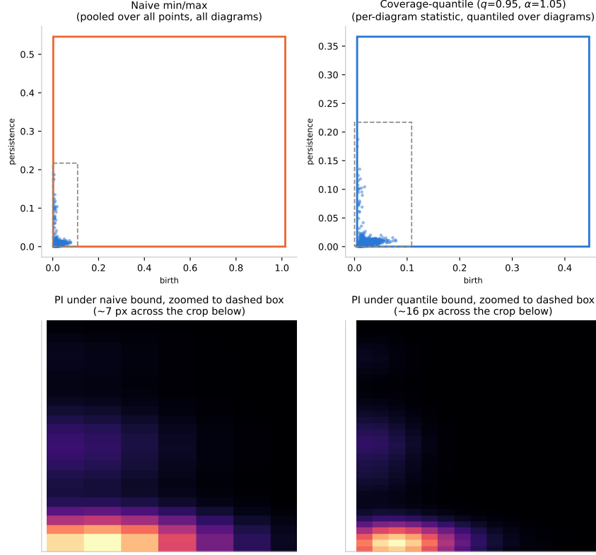
Figure 3: The same H_0 diagram (DTM filtration, k=5 – a plain Rips filtration gives every point birth 0, so the birth axis this figure calibrates would be degenerate) – the most feature-rich diagram among the non-outlier bulk (own max persistence at or below the 60th percentile), drawn from 2000 clouds sampled from the production Thomas design distribution (Section 5) – rendered under the naive pooled min/max bound (left) and the per-diagram coverage-quantile bound of q=0.95 , \alpha=1.05 (right). Top row: the diagram's own points against the calibrated birth-persistence box, with the dashed square marking the region zoomed into below; the naive box is stretched by a single high-offspring outlier diagram elsewhere in the population, not shown. Bottom row: the same physical region of birth-persistence space, rendered at each calibration's native pixel density – a 7 \times 7 block of mostly-fused pixels under the naive bound against a 16 \times 16 grid that keeps the secondary peak resolved under the quantile bound, since the same 64 \times 64 grid is stretched over a wider range.
