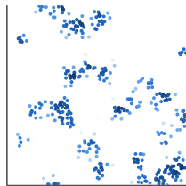
(a) Thomas, n=386 ; shade = \text{DTM}_5
