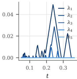
(g) landscape H_1 , K=5
