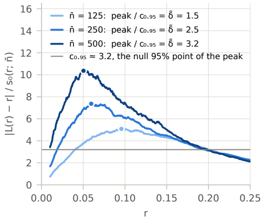
(b) One Thomas shape ( \mu = 2, s = 0.5 ), three \bar{n}
