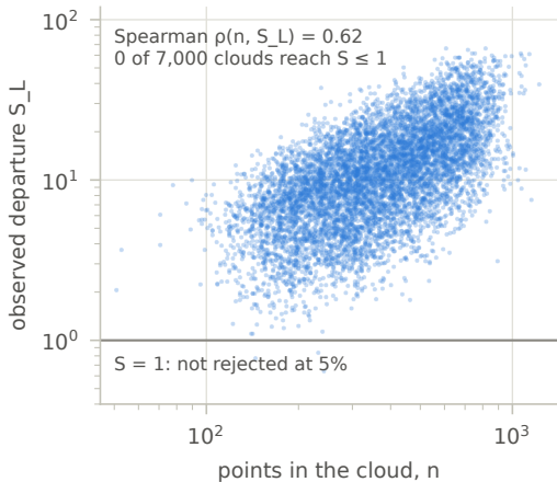
(a) DV1 Thomas: departure is tied to n
