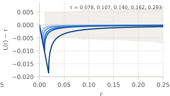
Matérn II: \tau \downarrow (one parameter)
