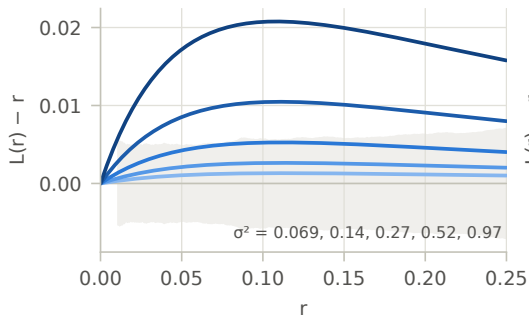
LGCP: \sigma^2 \downarrow at s/\tilde{n} = 1
