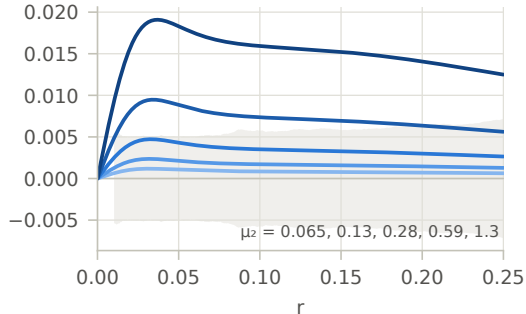
Nested: \mu_2 \downarrow at \mu_1 = 3, \rho = 6, s_2 = 0.2
