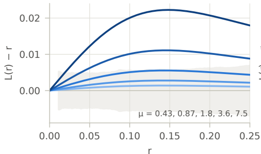
Thomas: \mu \downarrow at s = 1
