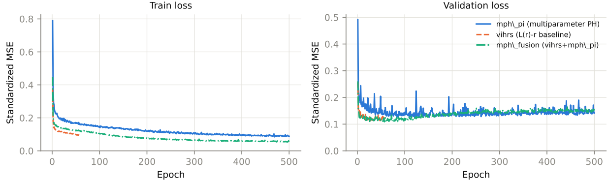
Figure 3: Training/validation loss curves, seed 9371 (representative).
