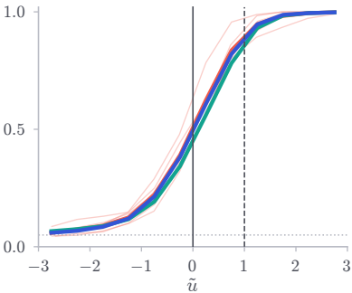
(a) Detection power
