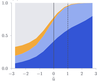
(b) ParamNet's call
