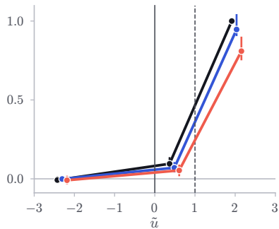
(c) Relative gain over CSR
