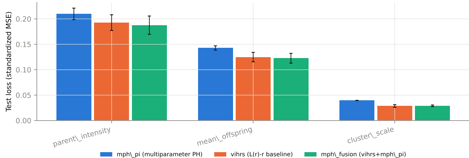
thomas: per-parameter test loss, mean \pm std over 3 seeds
