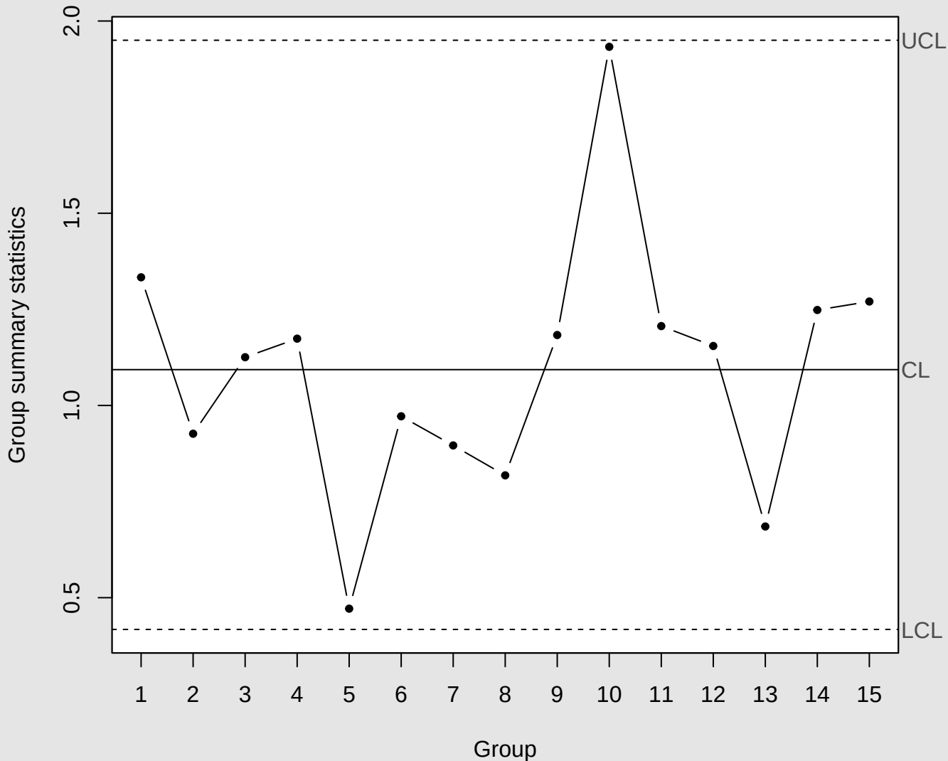
S Chart for x
