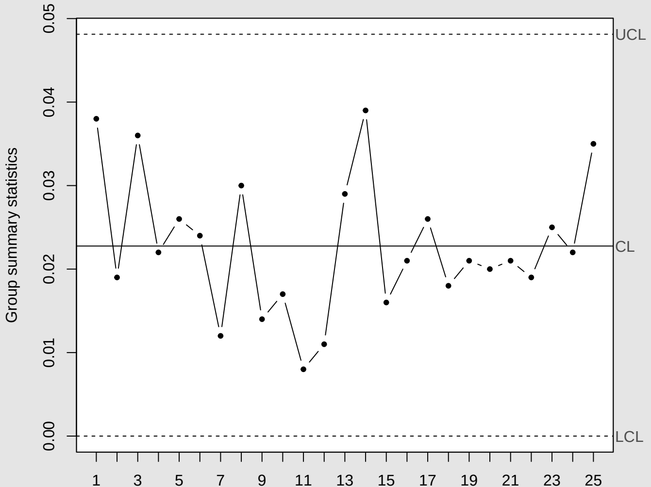
R Chart for x
