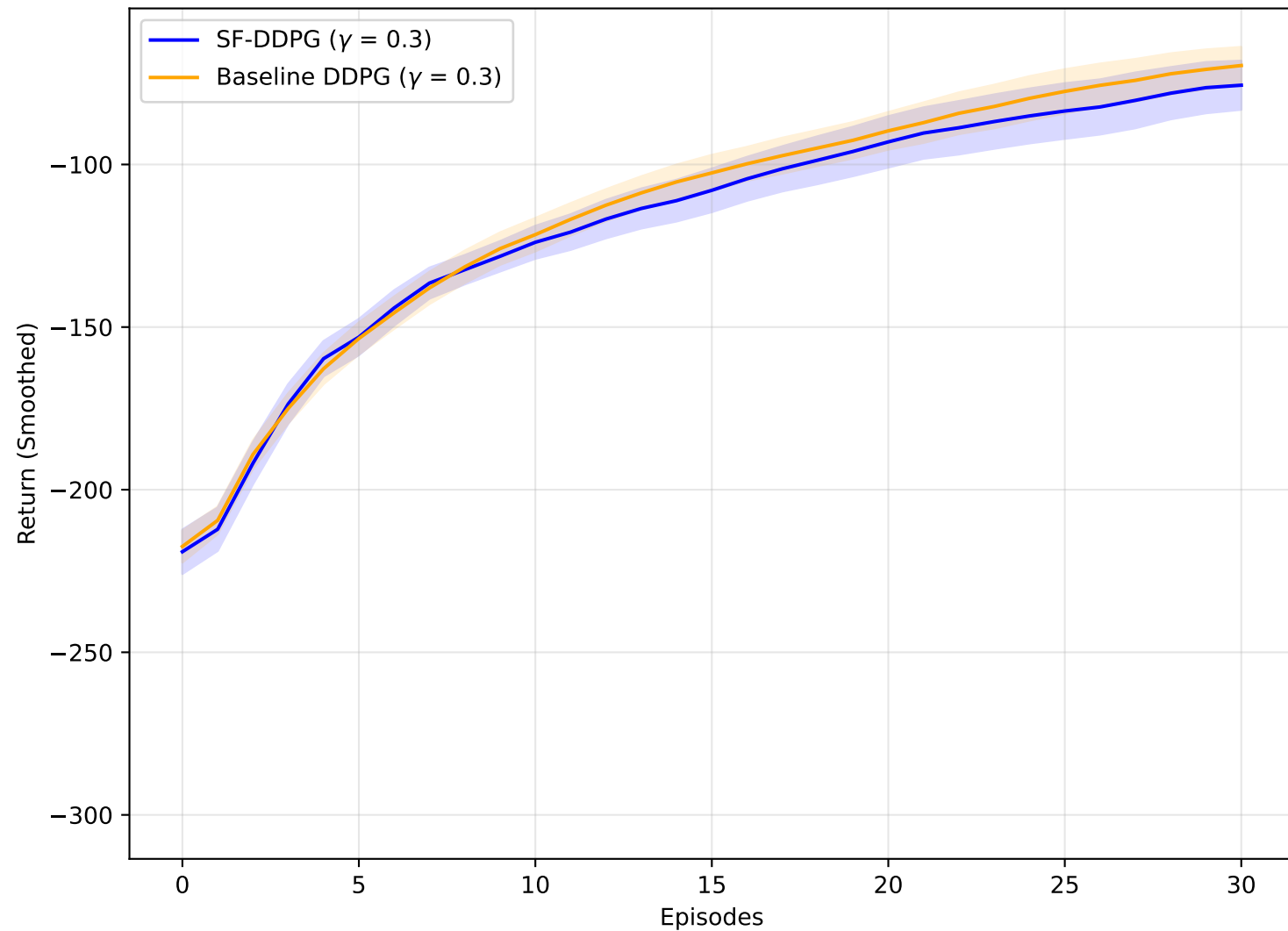
Phase 0: Task 1 (Forward)
