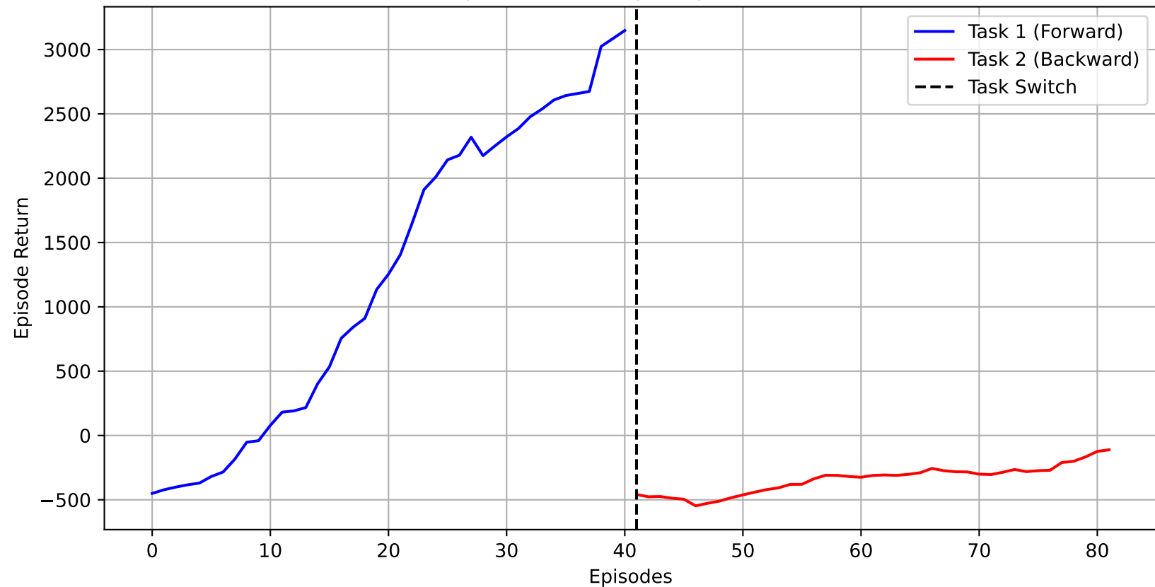
SF-DDPG Sequential Training Adaptation (HalfCheetah)
