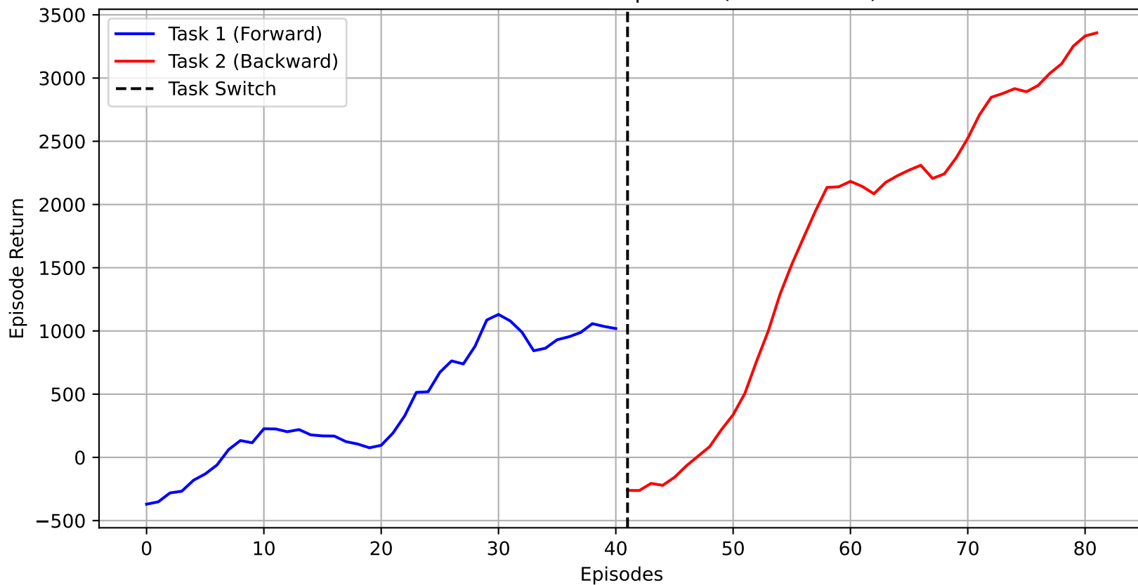
SF-DDPG Zero-Shot Adaptation (HalfCheetah)
