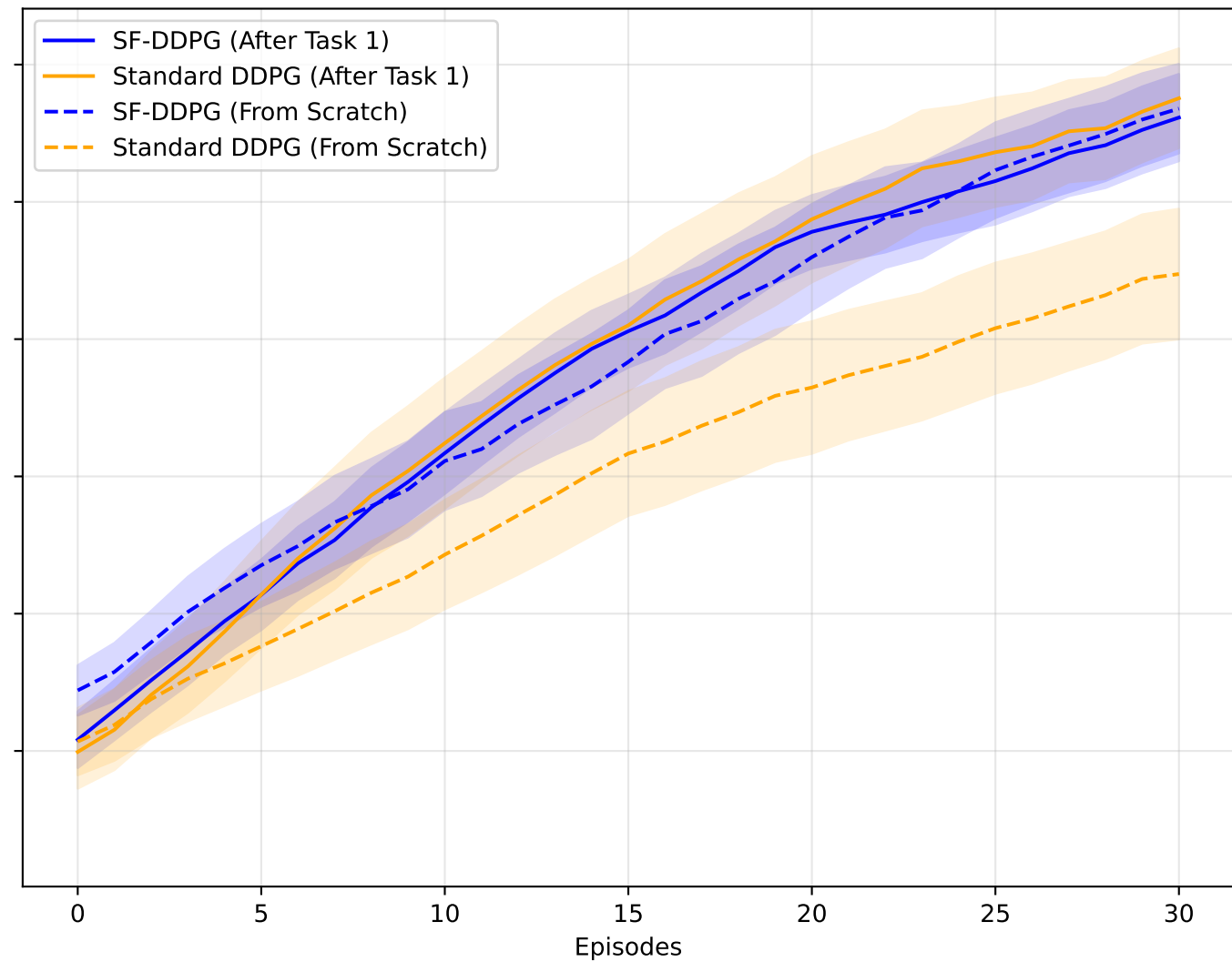
Task 2 (Backward) - Transfer vs Scratch, \gamma = 0.99
