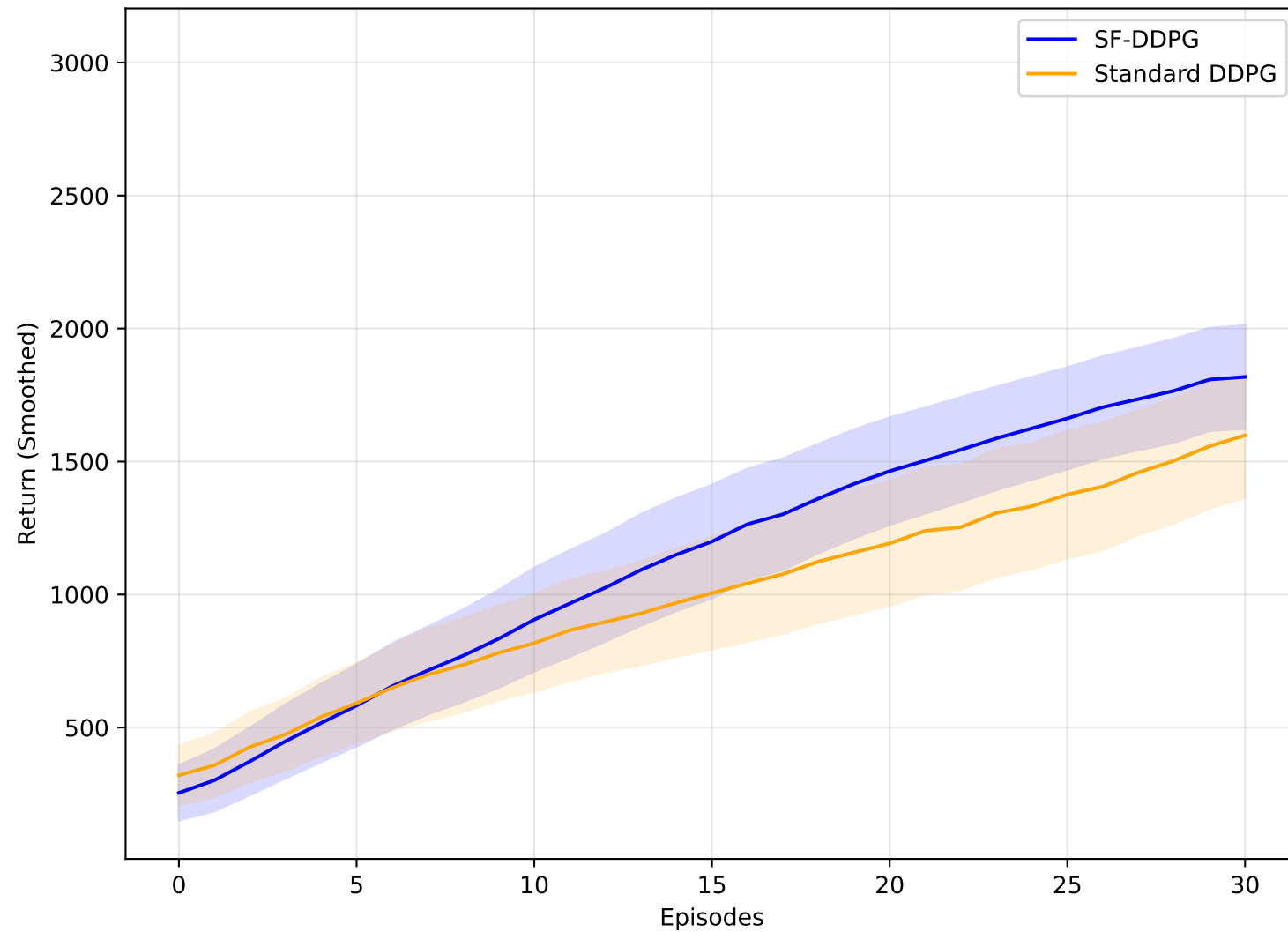
Task 1 (Forward), \gamma = 0.99
