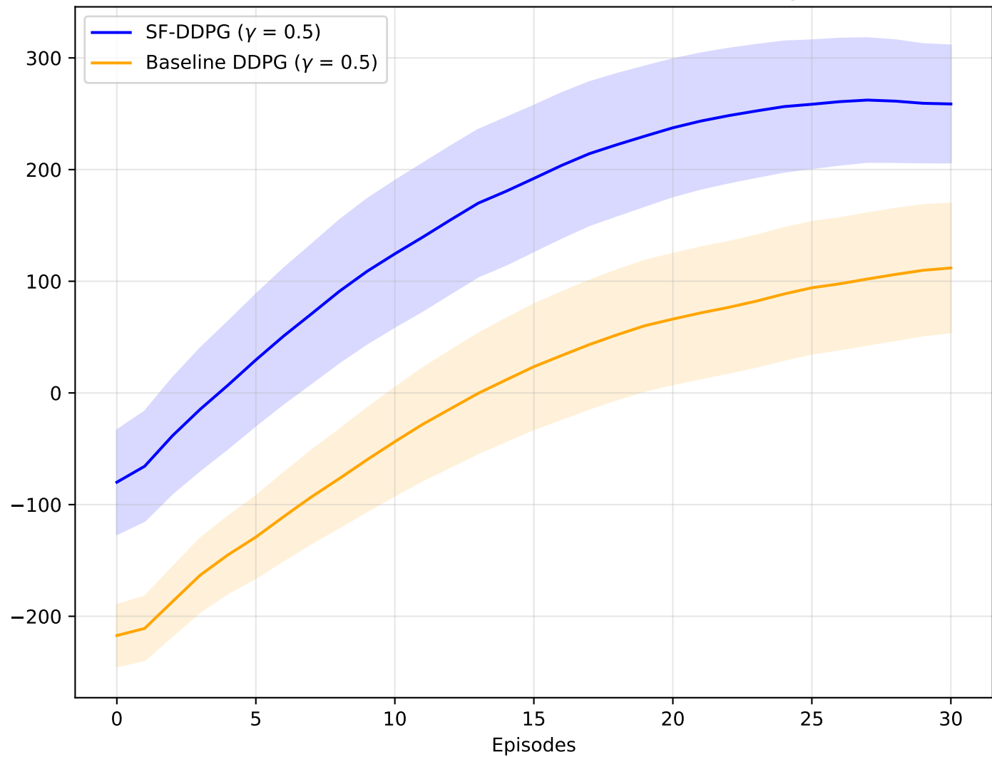
Phase 1: Task 2 (Backward) - Transfer Learning
