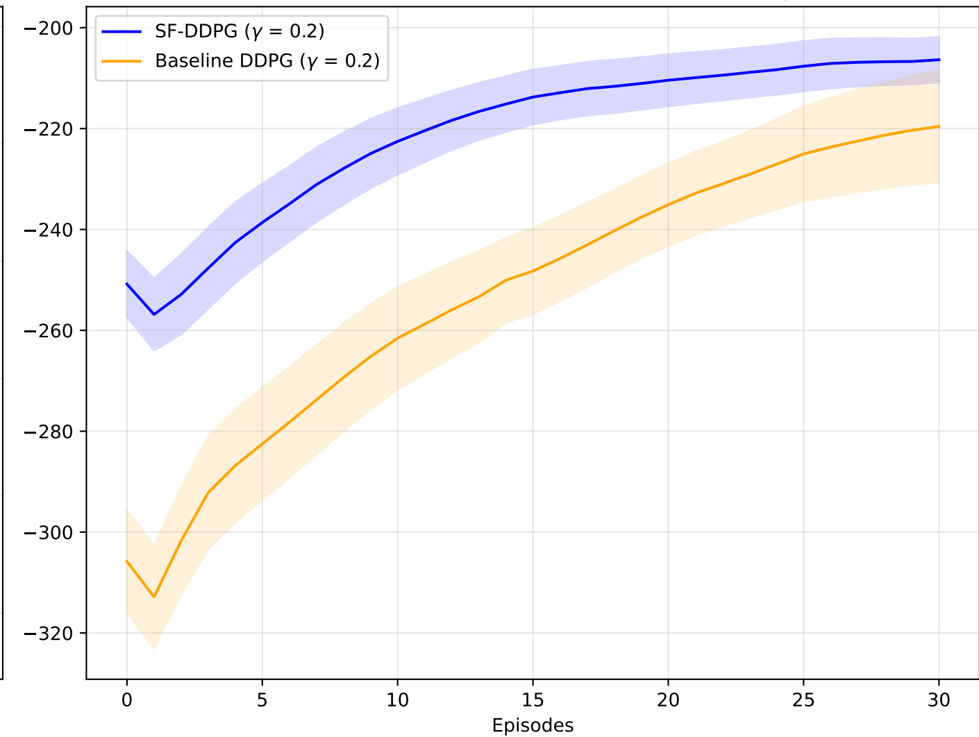
Phase 1: Task 2 (Backward) - Transfer Learning
