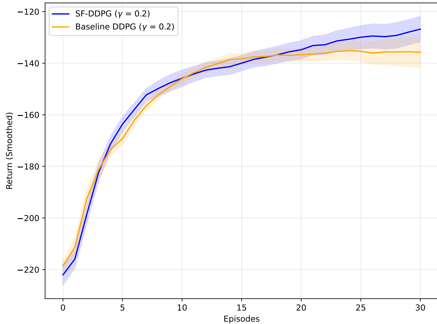
Phase 0: Task 1 (Forward)
