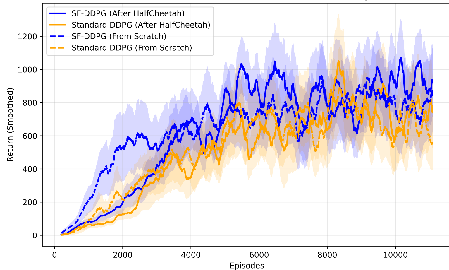
Phase 1: Walker2d Forward — Transfer vs Scratch, \gamma = 0.99
