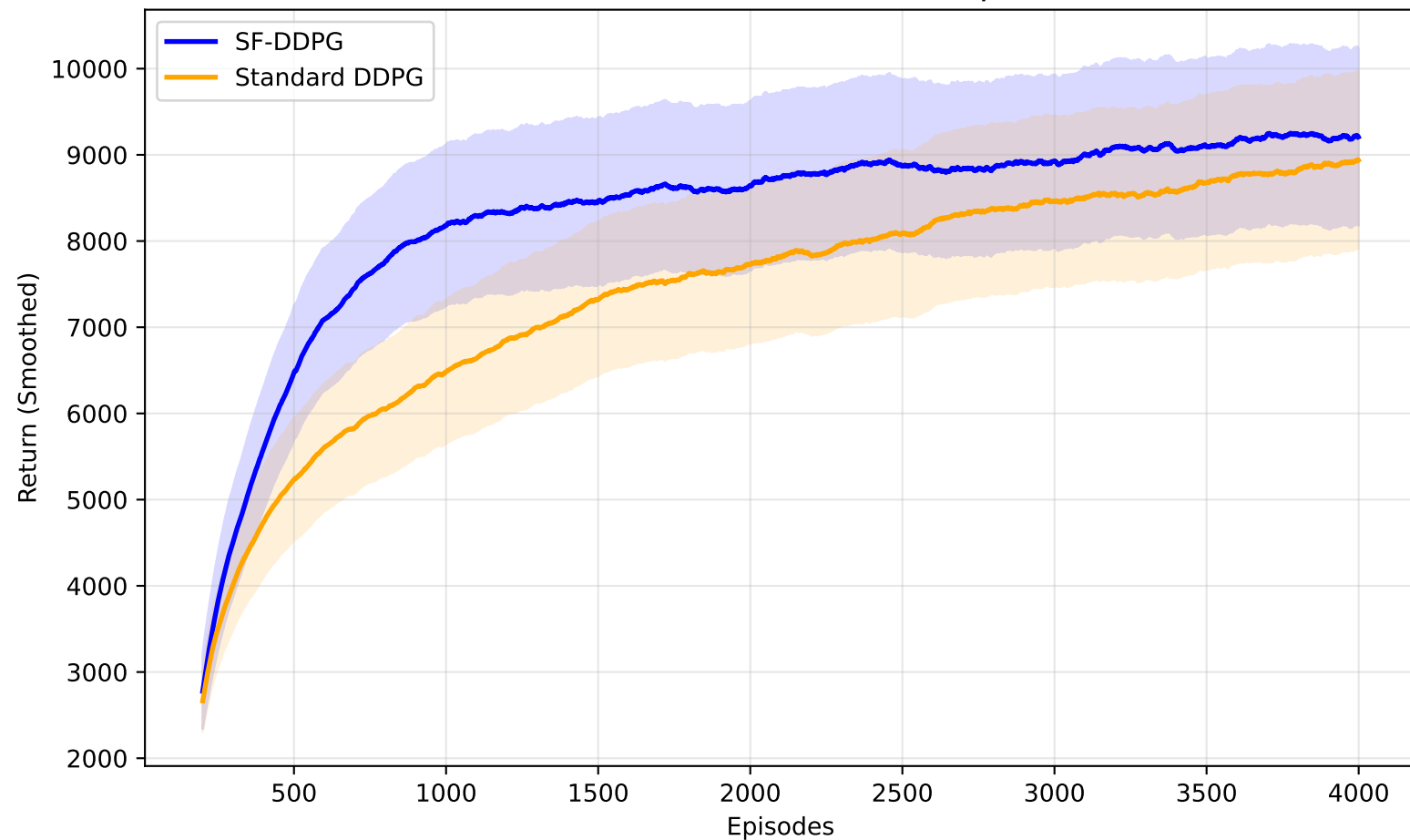
Phase 0: HalfCheetah Forward, \gamma = 0.99
