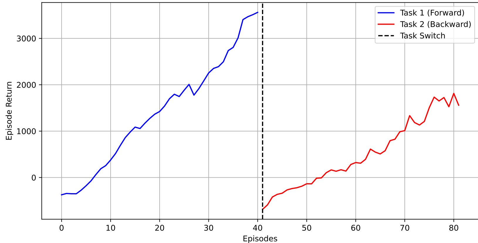
Standard DDPG Sequential Training Adaptation (HalfCheetah)
