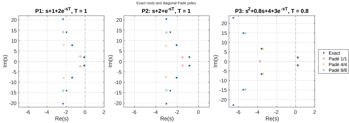
Figure 7.2: Roots of (7.1) (x) and poles of diagonal Padé models (o) at T = 1 (P1, P2) and T = 0.8 (P3). The exact chains continue to the left; the rational spectra are finite.
