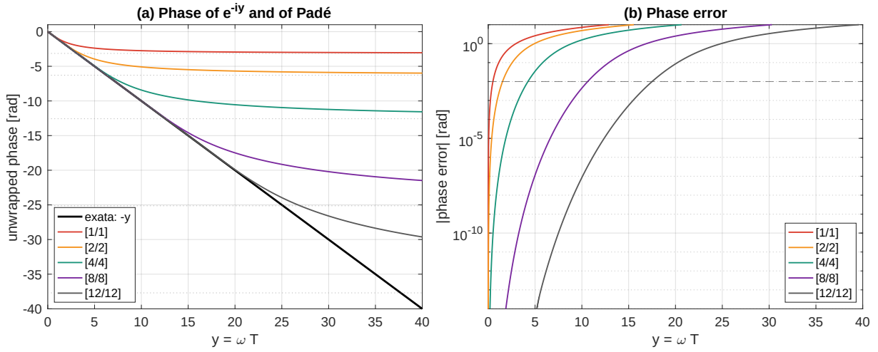
Figure 7.5: (a) Unwrapped phase of e^{-iy} and of [n/n] approximations; dotted lines mark -\pi . (b) Phase error; the dashed line marks 10^{-2} rad.
