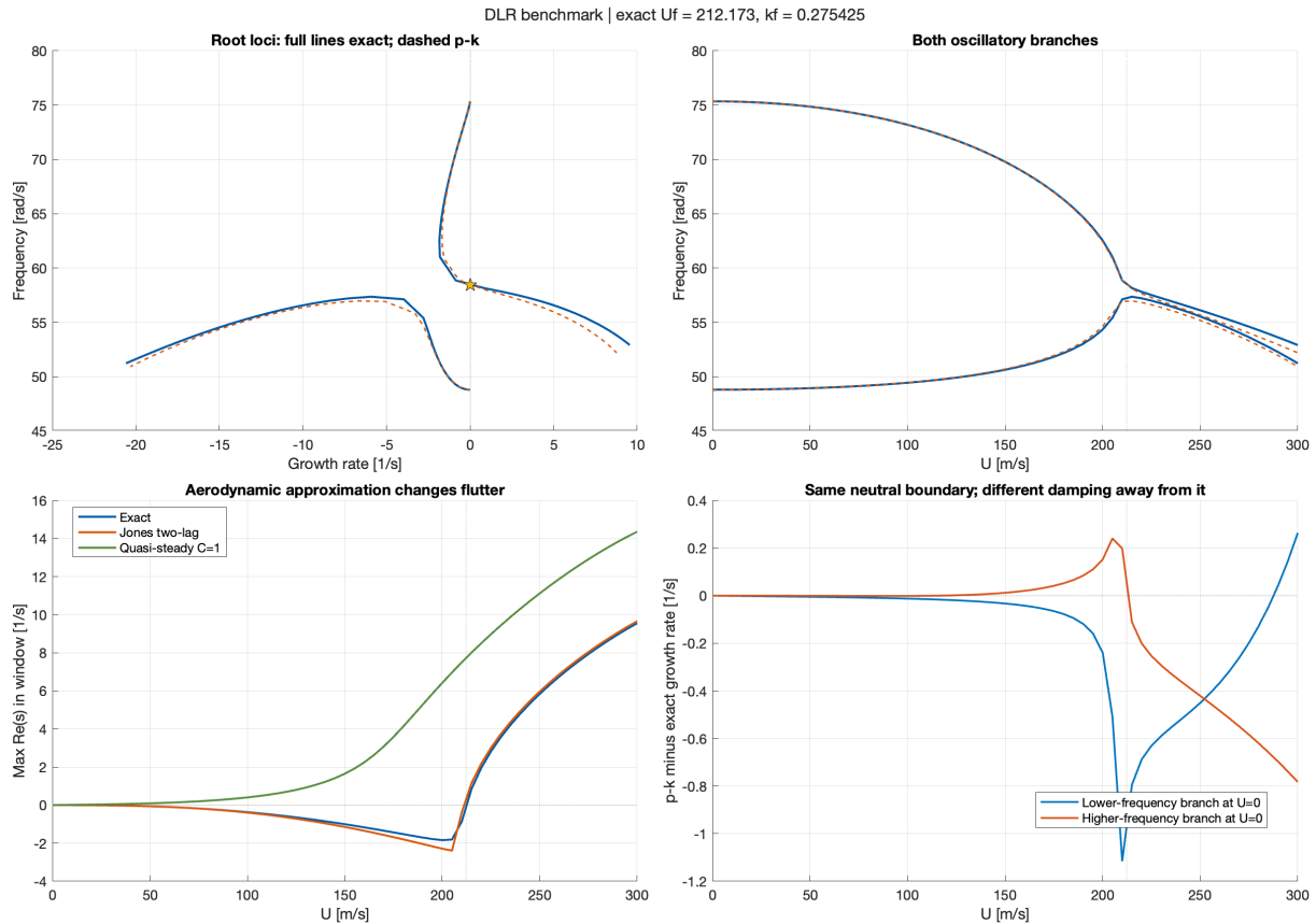
Figure 10.4: The dimensional benchmark of Kaiser and Quero [13], same layout as Figure 10.3.
