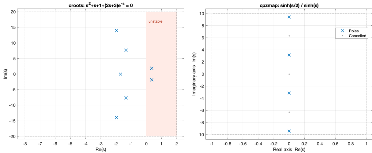
Figure 2.1: Left: roots of s^2 + s + 1 + (2s+3)e^{-s} in the rectangle [-8, 2] \times [-20, 20] (dashed); the shaded area is the right half-plane. Right: cpzmap of \sinh(s/2)/\sinh(s) ; grey dots are cancelled candidates.
