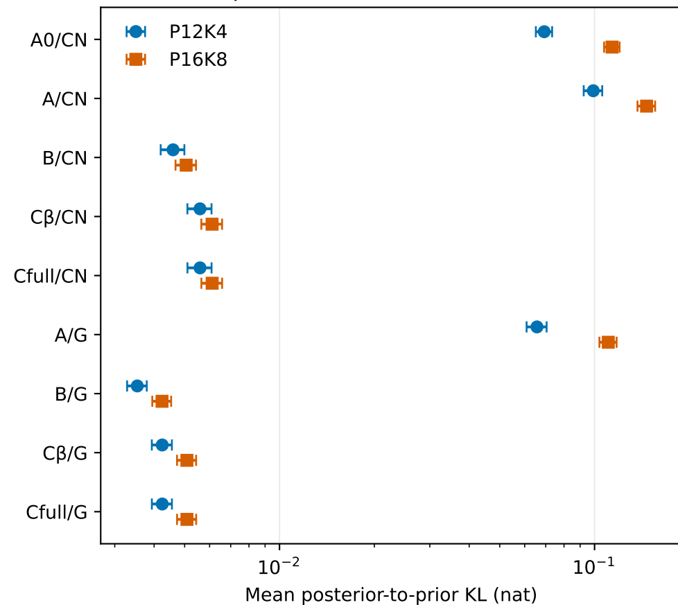
500 prior draws; error bars: \pm 1 MCSE
