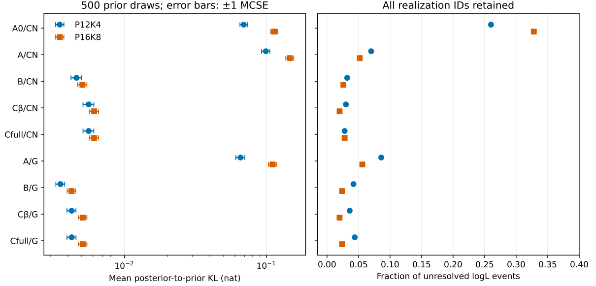
Figure 1: Prior-only information and numerical resolution in the completed campaign. Left: mean posterior-to-prior KL divergence, with one Monte Carlo standard error. Right: fraction of unresolved log-likelihood events among 500 prior draws. P12K4 and P16K8 are shown separately. Under approximate models, KL is descriptive rather than mutual information of the true generator.
