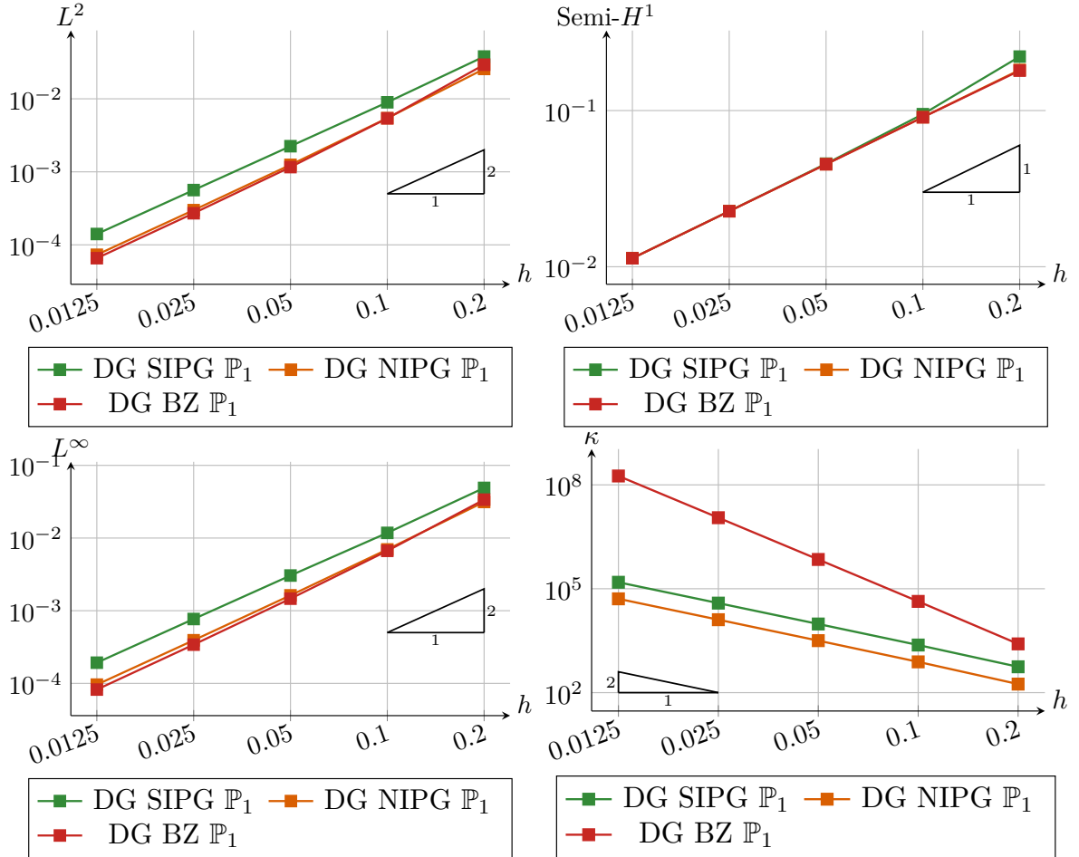
FIGURE 1 – Cas test 1.2.1, DG classique – n_{\text{cells}} \in \{5, 10, 20, 40, 80\} , n_b = 2 , n_{\text{quad}} = 3 .
