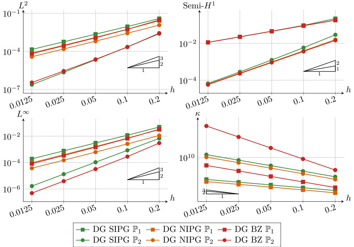
FIGURE 1 – Cas test 1.3.1, DG classique – n_{\text{cells}} \in \{5, 10, 20, 40, 80\} .
