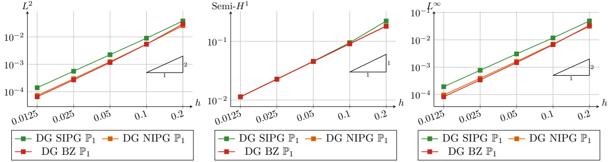
FIGURE 1 – Cas test 1.2.1, DG classique – n_{\text{cells}} \in \{5, 10, 20, 40, 80\} , n_b = 2 .
