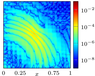
Absolute additive error |u - (u_\theta + C_h^+)|
