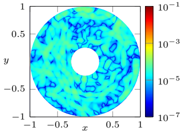
Absolute additive error |u - (u_\theta + C_h^+)|
