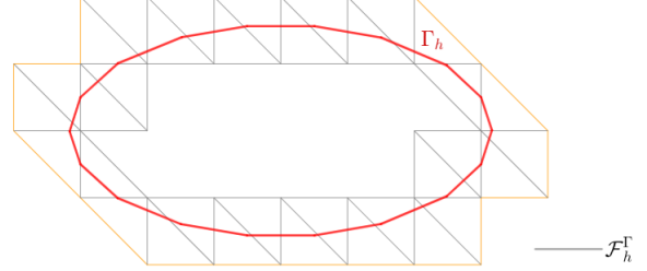
FIGURE 10 – Boundary edges.
