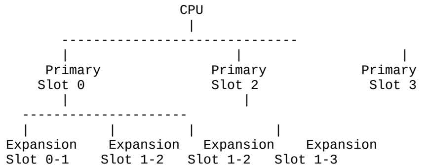
Fig. 2.2: MSX Slot Configuration (Part 1)
