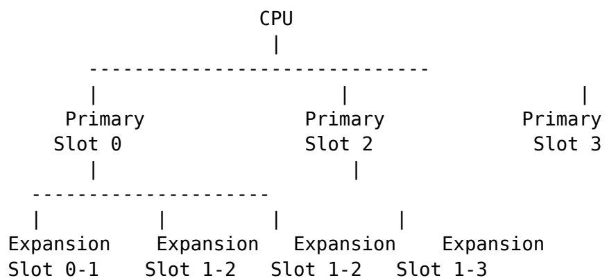
Fig. 2.2: MSX Slot Configuration (Part 1)
