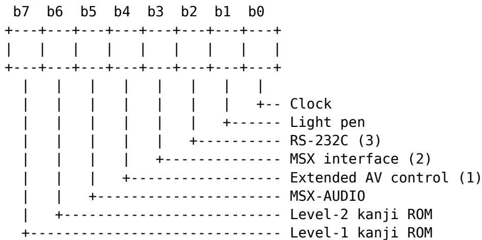
Figure 2.7: Device Enable
