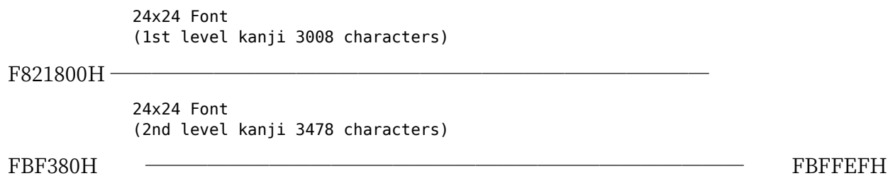
Figure 2-34 CGROM Address Map
