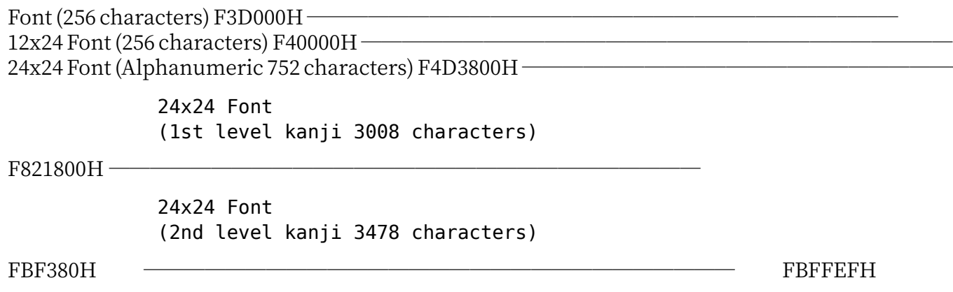
Figure 2-34 CGROM Address Map
