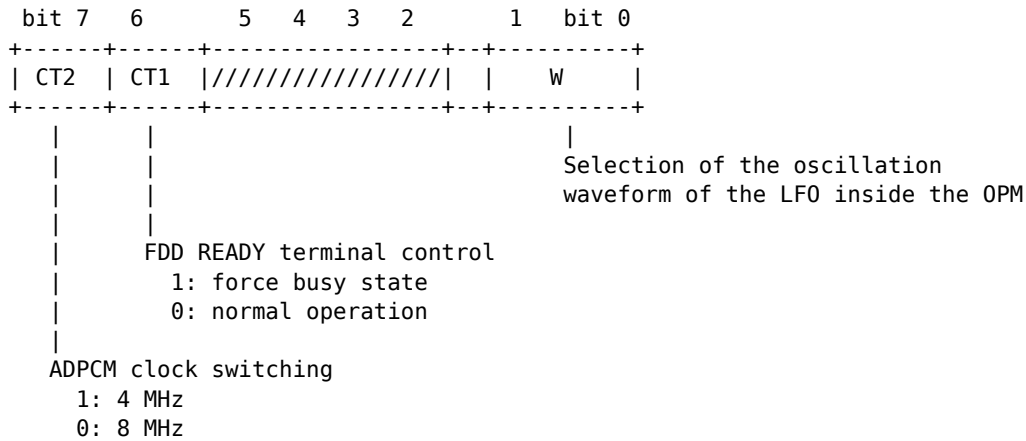
Fig. 38 OPM register (register No. = $1B)
