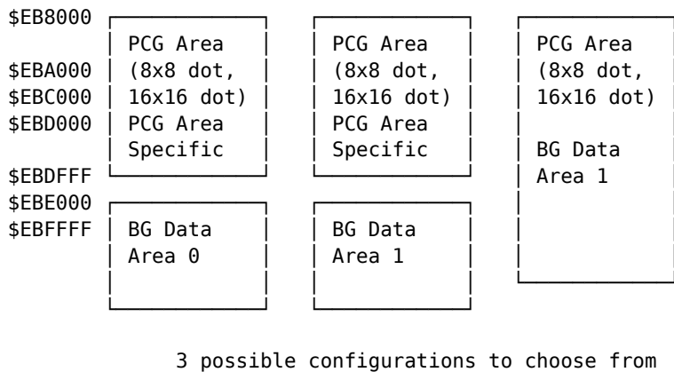
Diagram 7: PCG Area and BG Data Area Address Allocation
