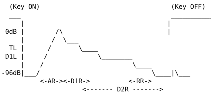
Fig. 31 Relationship between the envelope generator output waveform and the setting values
