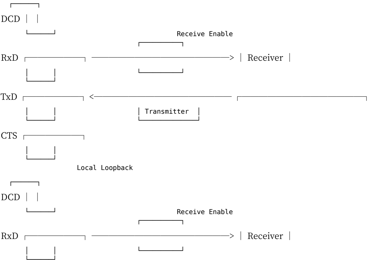
●Figure 10 Local Loopback and Auto Echo
