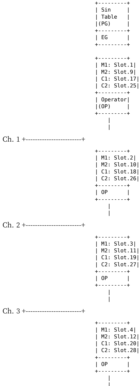
Each Slot Block Diagram
