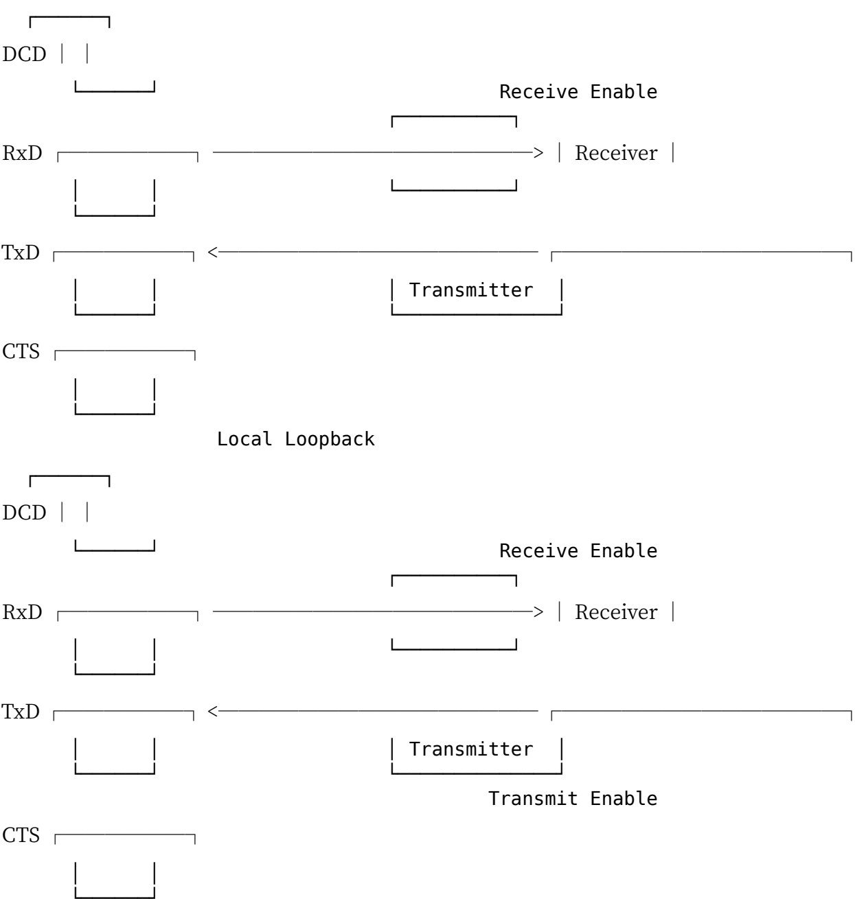
●Figure 10 Local Loopback and Auto Echo
