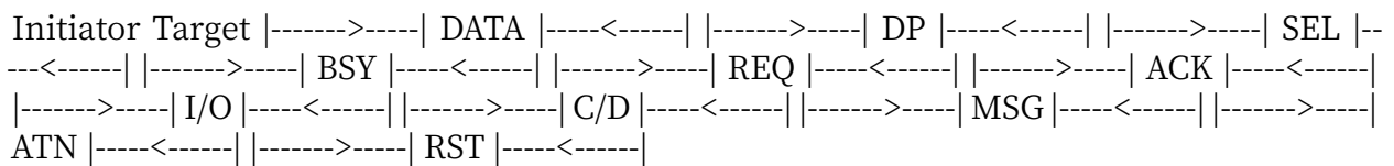
Fig ..... 2 SCSI Bus Signals
