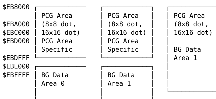
Diagram 7: PCG Area and BG Data Area Address Allocation
