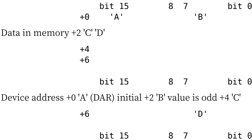
● Fig. 13 Transfer when the device port size is 8 bits
