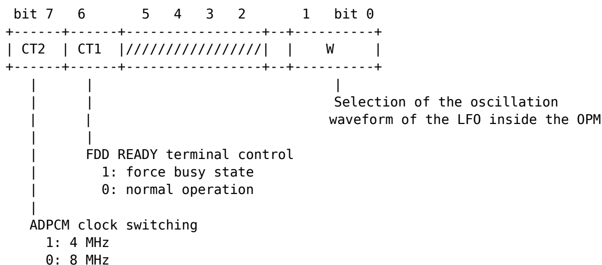
Fig. 38 OPM register (register No. = $1B)
