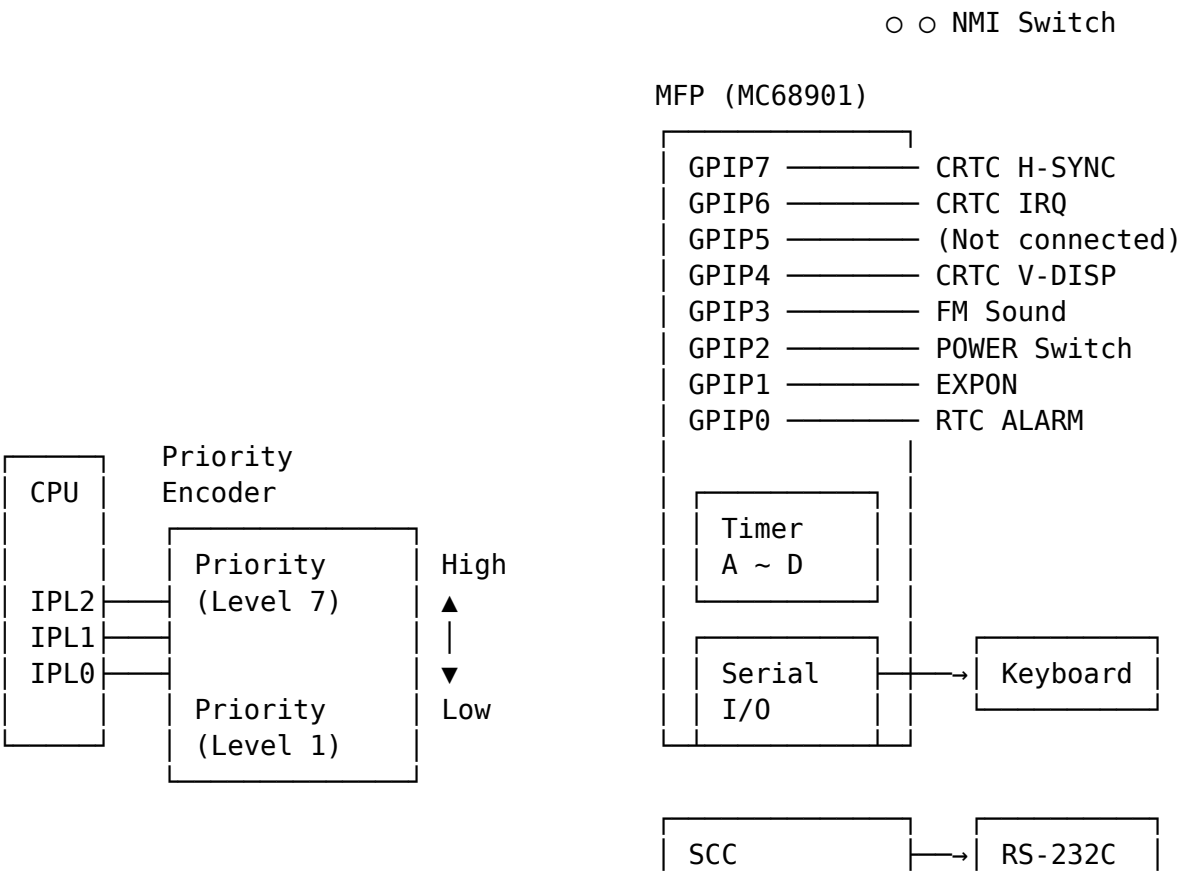
● Fig. 1 Interrupt System Diagram
