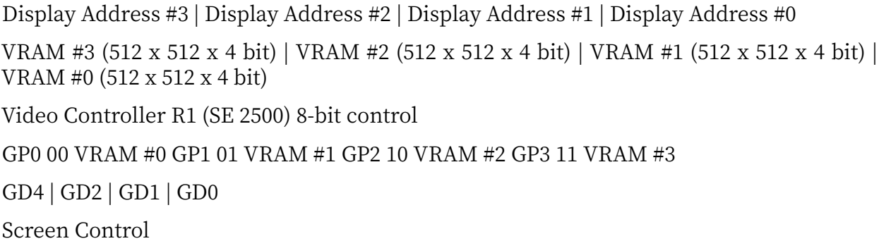
Figure: 20 Graphic Screen Inter-Priority Control Mechanism
