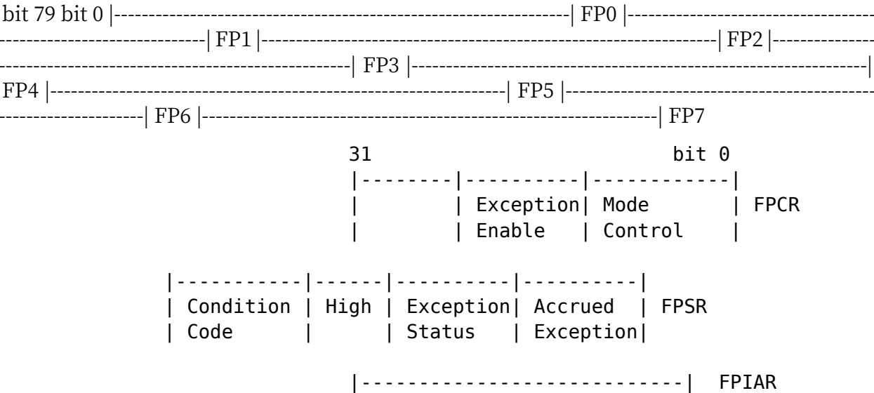
● Fig. 1 Internal Registers of the 68881
