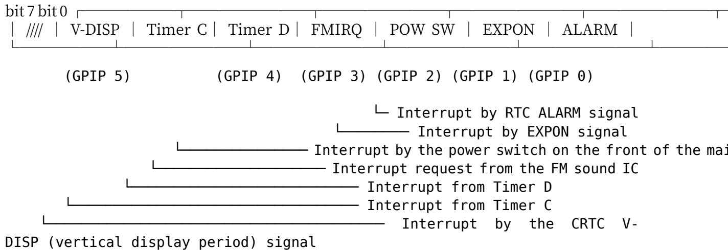
● Fig. 5 IERB, IPRB, ISRB, IMRB ($E88009, $E8800D, $E88011, $E88015)
