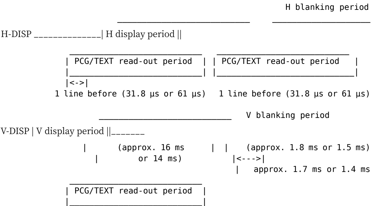
● Fig....E Register Read-out Timing
