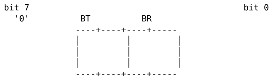
Figure ... 20 General Control Register (+$FF)
