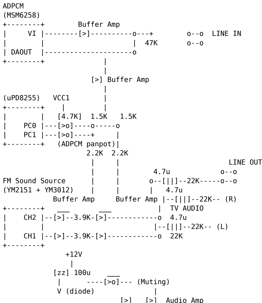
● Fig....1 Sound System Block Diagram
