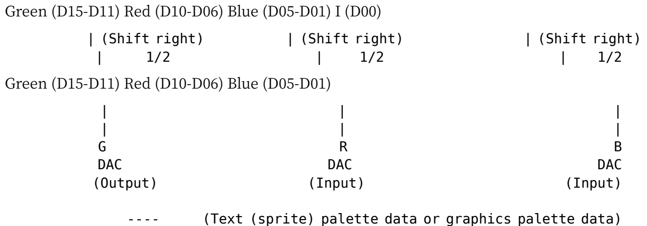
Figure 2-24 Transparent Mode
