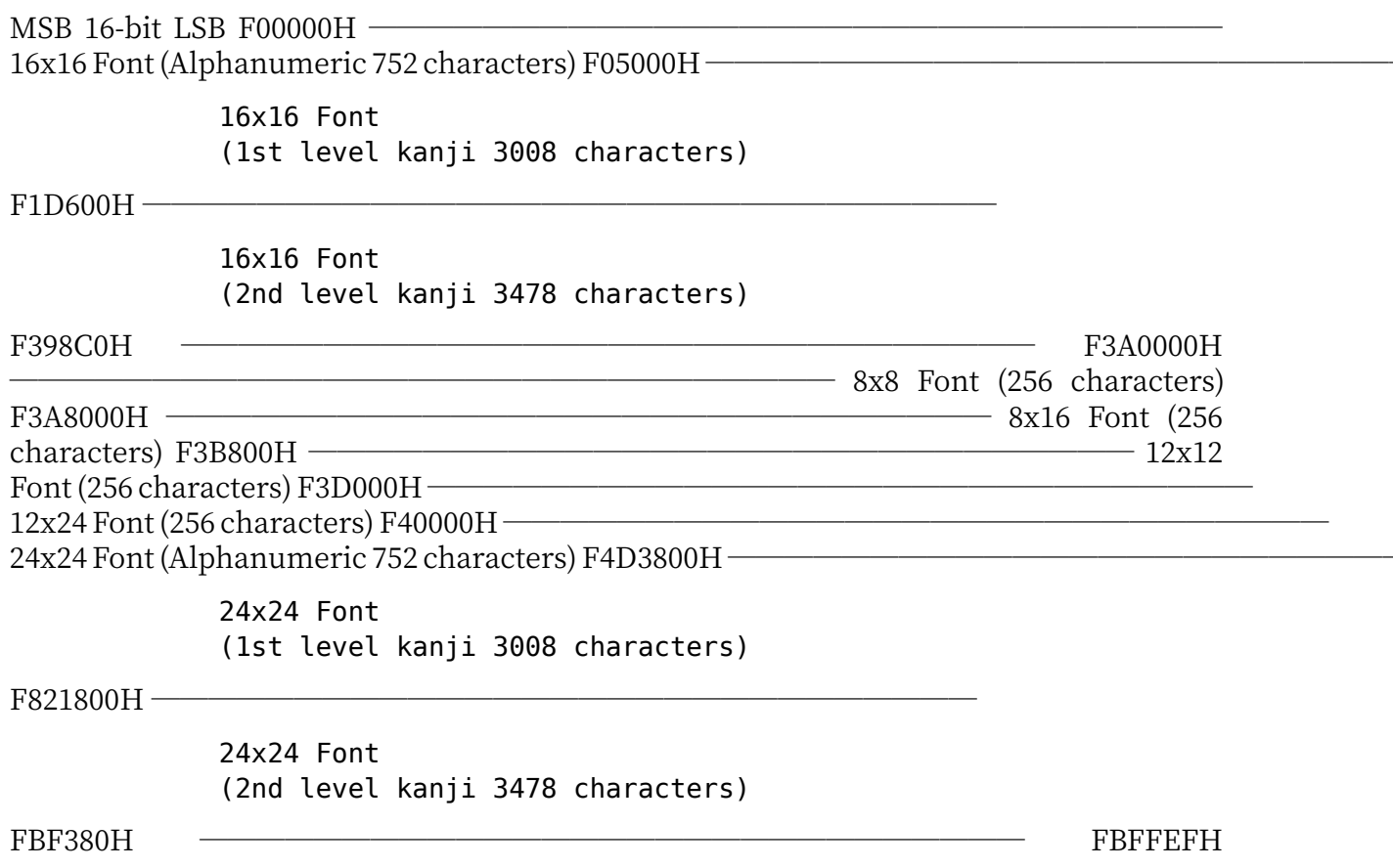
Figure 2-34 CGROM Address Map
