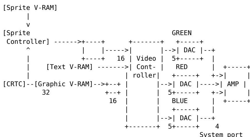
Fig. 4-1 Display control system block diagram
