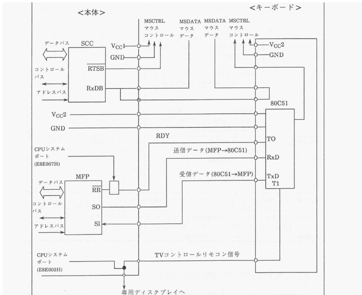
Figure 6-1 Keyboard and Mouse Surrounding Block Diagram
