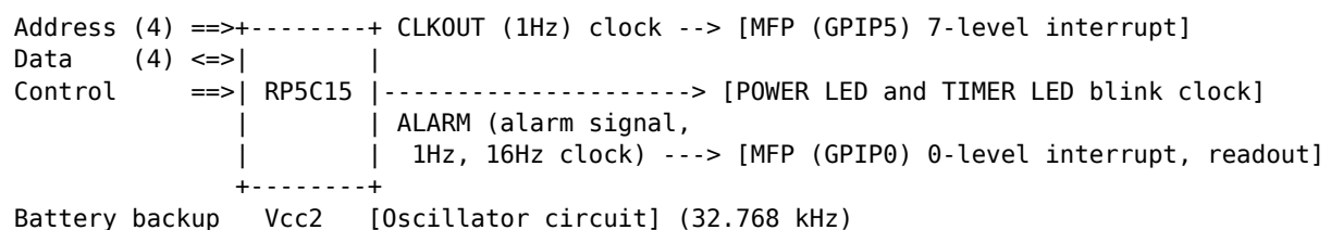
Figure 8-9 RTC Block Diagram
