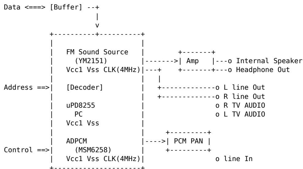
Figure 7-1 Sound System Block Diagram
