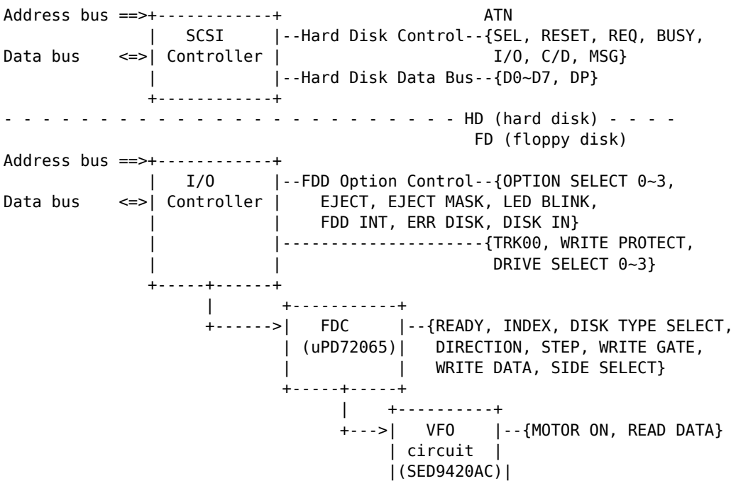
Figure 9-1 FDD/HDD Peripheral Block Diagram
